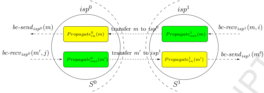
Fig. 4. Scheme of the interconnecting protocol.
