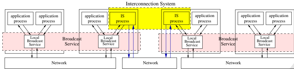
Fig. 2. Interconnection System.
